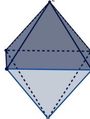
Octaedro
