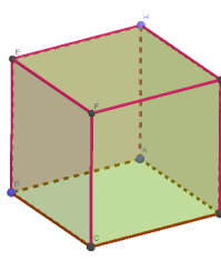
Hexaedro
